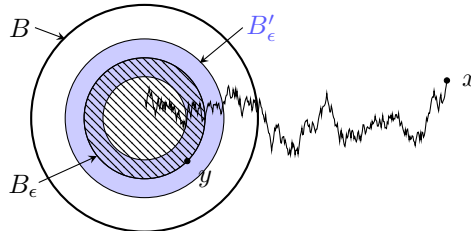
Figure 1: The big ball with thick boundary is B , the small, hatched ball is B_\epsilon and the shaded area denotes B'_\epsilon . The diffusion is started in x \in B^c .
