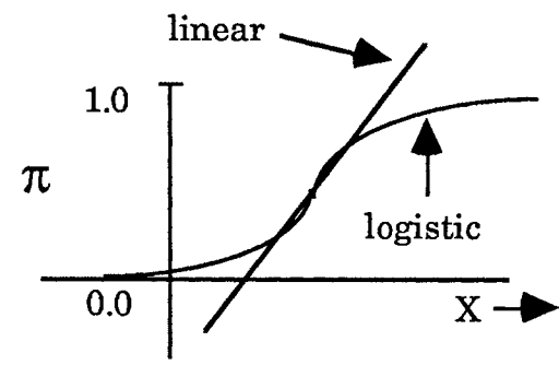
FIGURE 1. LINEAR VERSUS LOGISTIC FUNCTIONS OF X
