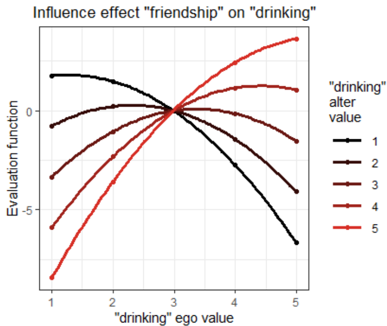
Figure 8: Plot of influence table for friendship with respect to drinking.
