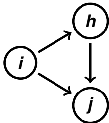
Transitive triplet (i, h, j)
