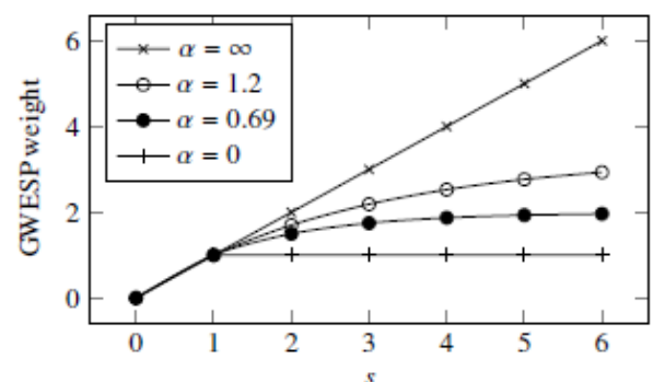
GWESP weight for a tie closing s two-paths for \alpha = \infty, 1.2, 0.69, 0 .
