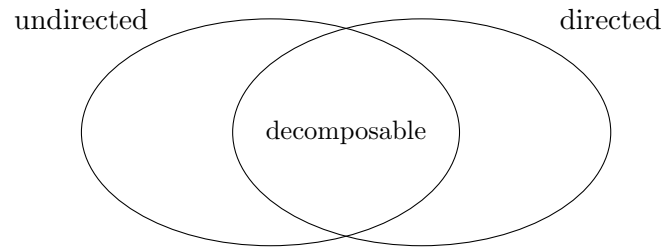
Figure 6.4: Venn diagram of model classes introduced by directed and undirected graphs.
