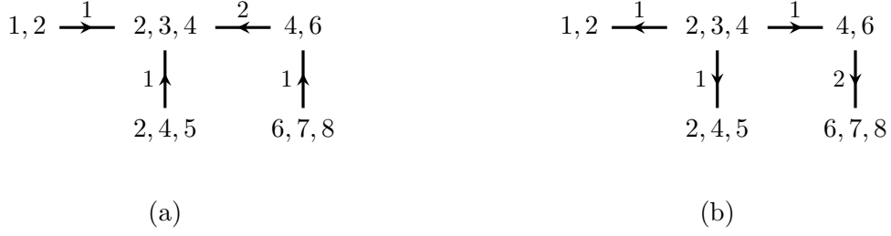
Figure 7.4: Illustration of the junction tree algorithm with \{2, 3, 4\} chosen as the root. (a) Collect steps towards the root: note that the \{4, 6\} to \{2, 3, 4\} step must happen after the \{6, 7, 8\} to \{4, 6\} update. (b) Distribute steps away from the root and towards the leaves: this time the constraint on the ordering is reversed.
