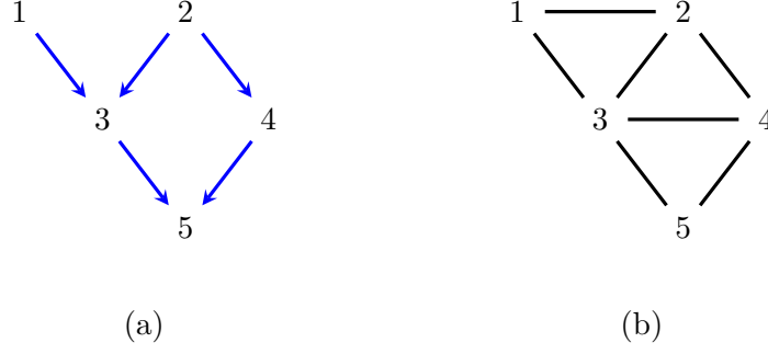
Figure 6.2: (a) A directed graph and (b) its moral graph.
