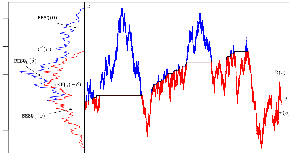
Figure 7: This figure is from [43], showing the Brownian motion split along the increasing path \gamma\ell_\gamma , with the positive excursions of X_\gamma in blue, above the increasing path, and the negative excursions of X_\gamma in red, below the increasing path. The construction is stopped at \tau(v) , when the inverse local time of Brownian motion at level 0 exceeds v > 0 . The left-hand side of the figure shows the total Brownian local times (up to time \tau(v) ), split according to the red and blue contributions, and identified as squared Bessel processes of dimensions \delta , -\delta and 0, where \delta = 2\alpha .
