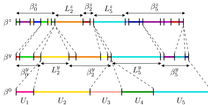
Figure 1: Illustration of the transition kernel \kappa_y^{\alpha, \theta} . The initial state \beta^0 has five blocks: U_1, \dots, U_5 . Some contribute \emptyset for time y , here U_1, U_3 and U_4 . The others each contribute a leftmost block L_j^y and a partition \beta_j^y = G_j \bar{\beta}_j of further blocks. If we add “immigration” \beta_0^y = G^y \bar{\beta}_0 , then \beta^y = \beta_0^y \star (0, L_2^y) \star \beta_2^y \star (0, L_5^y) \star \beta_5^y . The semigroup property requires consistency of a transition from 0 to z and composition of the transitions from 0 to y and from y to z .
