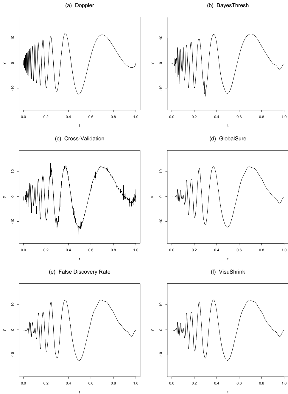
Figure 8: (a) Doppler function; various reconstructions based on 1024 equally-spaced values of the function with the addition of independent N(0, \sigma^2) noise with \sigma = 7/3 (RSNR = 3): (b) BayesThresh ( \alpha = 0.5 , \beta = 1 ); (c) Cross-Validation ; (d) GlobalSure ; (e) False Discovery Rate ; (f) VisuShrink .
