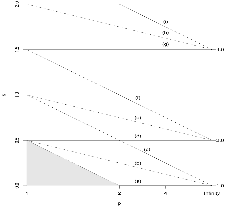
Figure 3: The critical values of the Besov space parameters s and p for certain values of \alpha and \beta for any values of 1 \leq q \leq \infty . The values of \alpha = 1, 2 and 4 are indicated on the right hand axis. The values of \beta are indicated by the line style (solid: \beta = 0 ; dotted: \beta = 0.5 ; dashed: \beta = 1 ). For each value (\alpha, \beta) , realizations lie in all Besov spaces with parameter values below the line plotted. They also lie in spaces on the critical line if 0 \leq \beta < 1 , 1 \leq p < \infty and q = \infty . The shaded region represents the range of (p, s) excluded by the conditions of Theorem 1. The p -axis is transformed to be linear in (1 - 1/p) . Labels (a)-(i) correspond to the realizations given in Figure 2.
