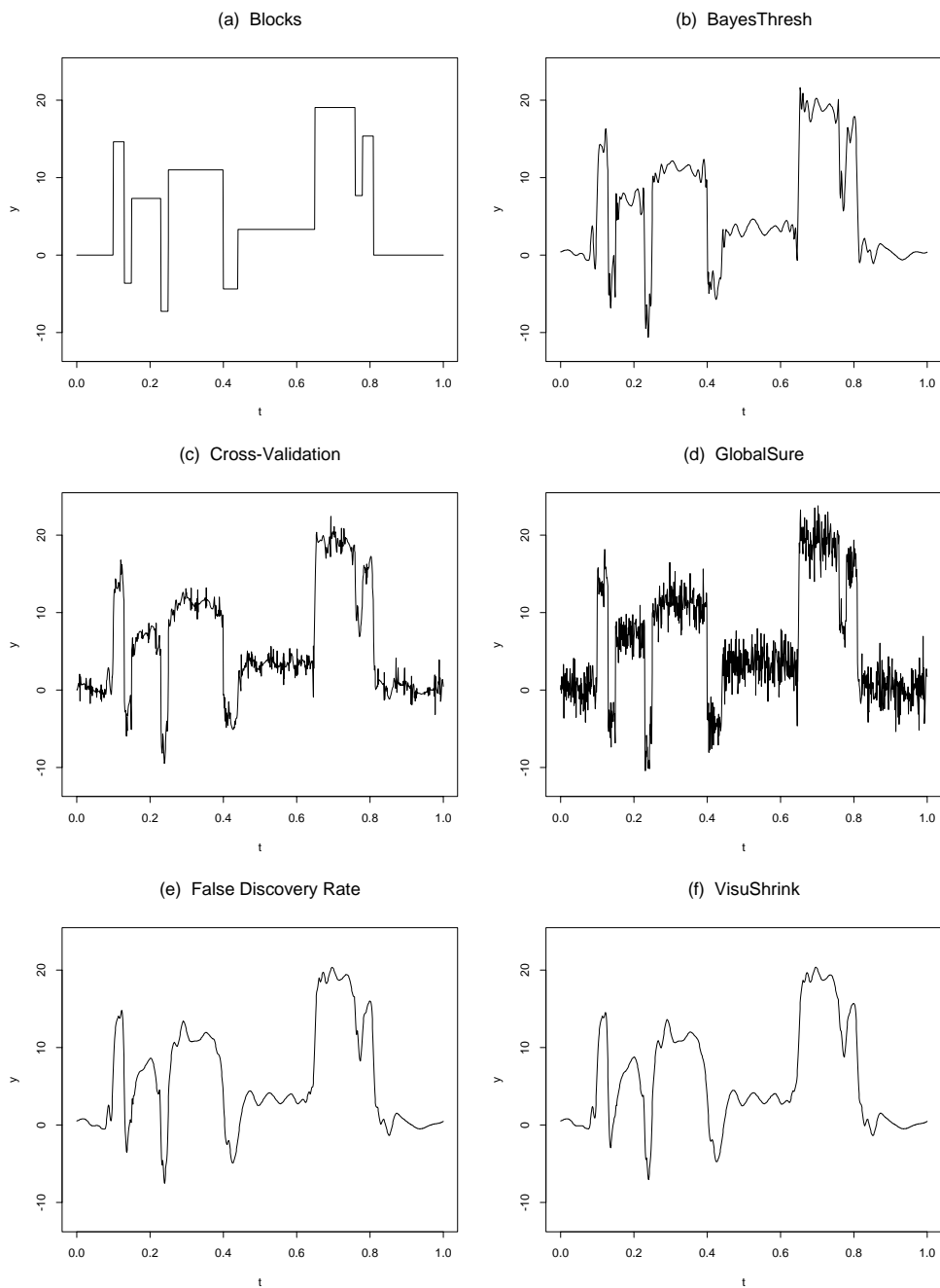
Figure 5: (a) Blocks function; various reconstructions based on 1024 equally-spaced values of the function with the addition of independent N(0, \sigma^2) noise with \sigma = 7/3 (RSNR = 3): (b) BayesThresh ( \alpha = 0.5 , \beta = 1 ); (c) Cross-Validation ; (d) GlobalSure ; (e) False Discovery Rate ; (f) VisuShrink .
