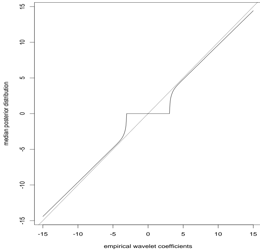
Figure 1: The median of posterior distribution (solid line) as function of the empirical wavelet coefficients. Hyperparameters were chosen as \tau^2 = 25 , \pi = 0.05 , while \sigma was fixed at 1. (The dotted line shows the diagonal.)
