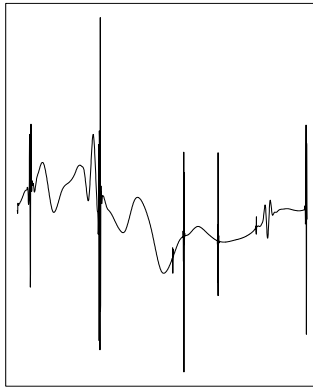
Figure 4: A realization with hyperparameters \alpha = 0.5 , \beta = 1 , with n = 2048 , C_1 = 1 and C_2 = 2 .
