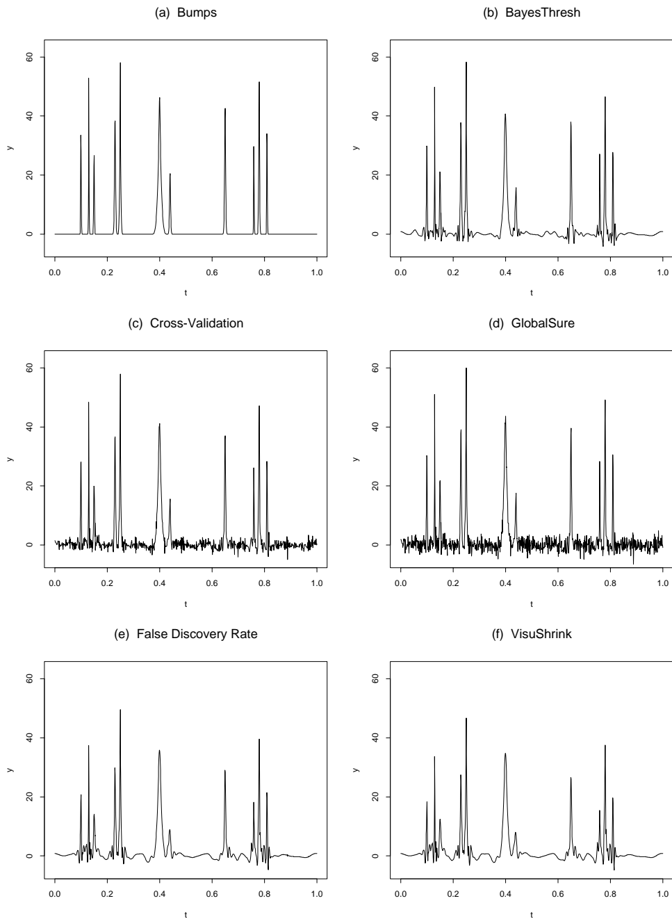
Figure 6: (a) Bumps function; various reconstructions based on 1024 equally-spaced values of the function with the addition of independent N(0, \sigma^2) noise with \sigma = 7/3 (RSNR = 3): (b) BayesThresh ( \alpha = 0.5 , \beta = 1 ); (c) Cross-Validation ; (d) GlobalSure ; (e) False Discovery Rate ; (f) VisuShrink .
