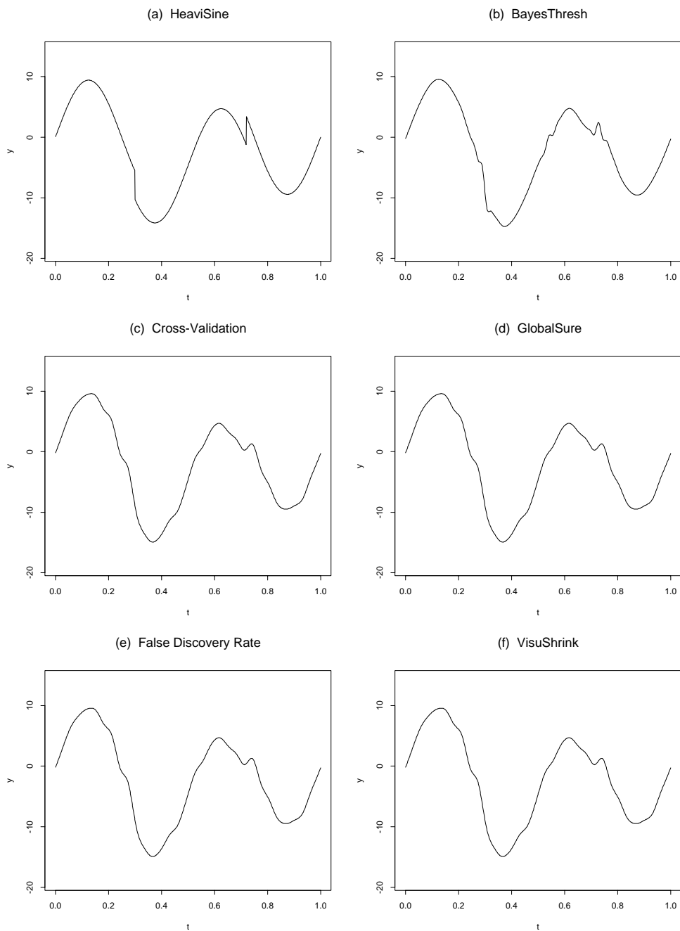
Figure 7: (a) HeaviSine function; various reconstructions based on 1024 equally-spaced values of the function with the addition of independent N(0, \sigma^2) noise with \sigma = 7/3 (RSNR = 3): (b) BayesThresh ( \alpha = 0.5 , \beta = 1 ); (c) Cross-Validation ; (d) GlobalSure ; (e) False Discovery Rate ; (f) VisuShrink .
