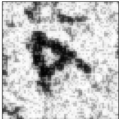
post mean
