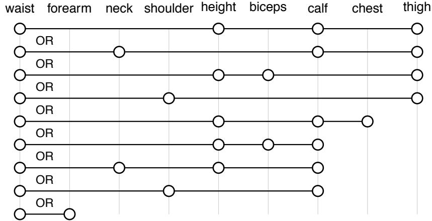
Figure 2: An alternative presentation of the results in the regression example. All dots on each horizontal line form a set of hypotheses. Out of all nine sets, at least one must correspond to a set of false null hypotheses (conditional on event E ).
