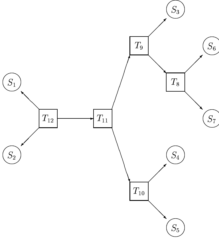
Figure 2: A tree with seven observed sequences.
