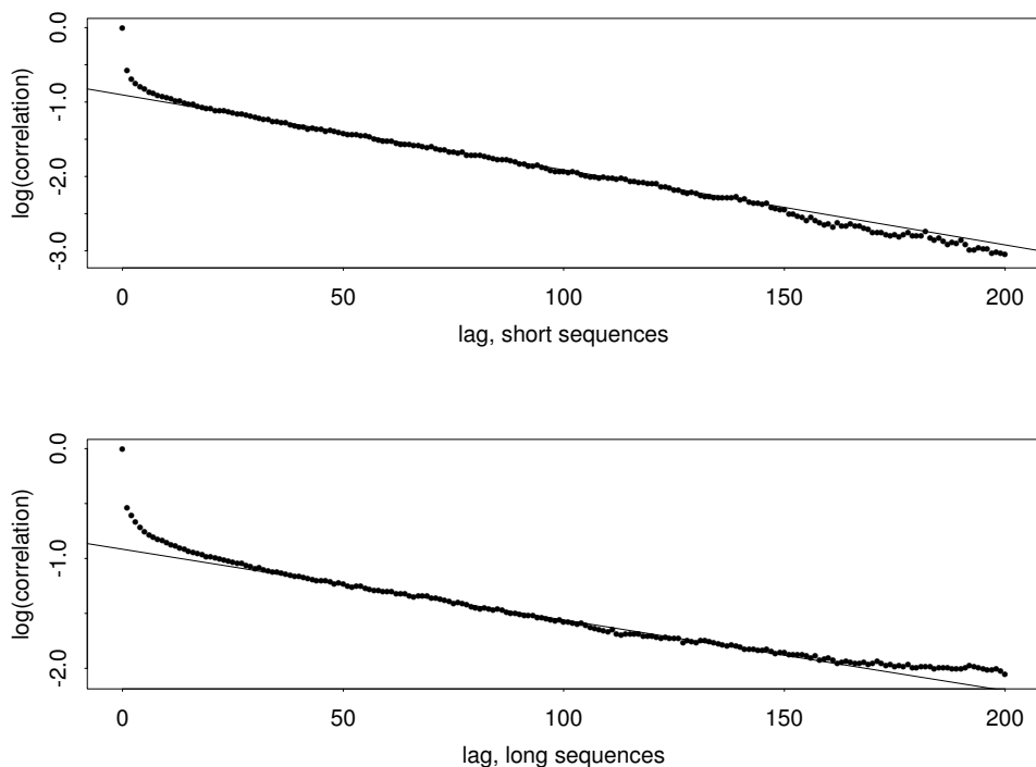
Figure 3: Log of autocorrelations for the number of deletions along branch 2.
