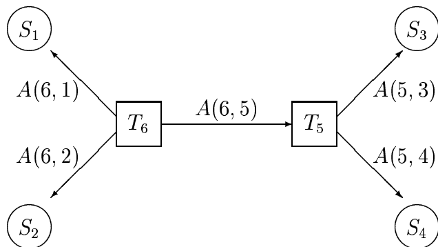
Figure 1: A tree with four observed sequences.
