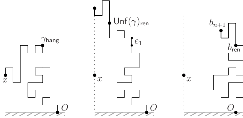
FIGURE 3. Left: A walk \gamma \in \text{SAHSW}_n ending at x . Middle: The unfolding of \gamma , \text{Unf}(\gamma) , and its last renewal point \text{Unf}(\gamma)_{\text{ren}} . Notice the bold edge e_1 added between \gamma^1 and the reflection of \gamma^2 . Right: A walk b \in \Phi(\gamma) . Its last renewal point is b_{\text{ren}} ; b[0, \text{ren}] is a bridge and b[\text{ren}, n+1] is equal up to translation to \text{Unf}(\gamma)[\text{ren}, n+1] (bold). The choice of b[0, \text{ren}] may be such that \pi_1(b_{n+1}) \neq \pi_1(x) .
