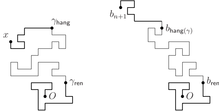
FIGURE 4. Left: A walk \gamma \in E_M(x) . Right: A walk b \in \Phi(\gamma) . The first and last parts of b (bold) are the same as those of \gamma (up to translation and reflection). Its middle part is a bridge with appropriate length and e_1 -displacement.
