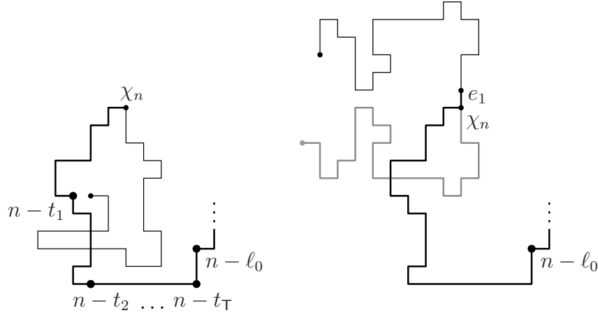
FIGURE 7. Left: The final portion of \chi in bold, and a walk contained in C_1 and in A_1 but not in A_2 . Right: A walk \gamma \in W \setminus A (gray) may be reflected and added to \chi^{\ell_0} (black) to create a walk starting with \chi^{\ell_0} , with hanging point different from \chi_n . When concatenating \mathcal{R}_{\chi_n}(\gamma) to \chi^{\ell_0} , an extra vertical edge is added in to ensure non-intersection, and the last edge is deleted to preserve length n .
