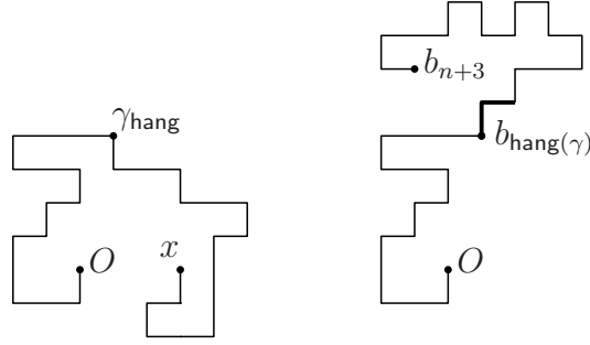
FIGURE 5. Left: A self-avoiding walk \gamma \in F_j . Right: A walk b \in \Phi(\gamma) . The point b_{\text{hang}(\gamma)} is the (j+1) -st z -renewal point of b ; it is followed by the edges e_1, e_2 (in bold), then by a half-space walk of length n - \text{hang} + 1 .
