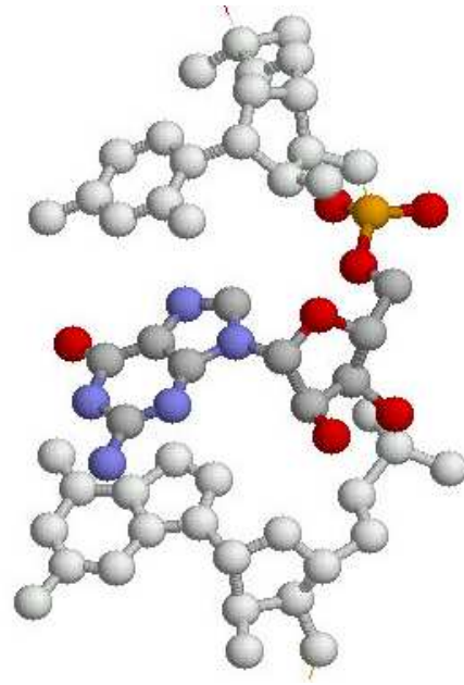
Guanine
