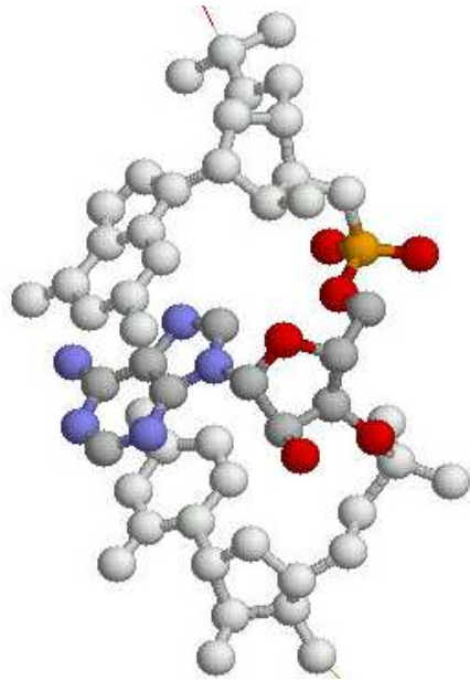
Adenine
