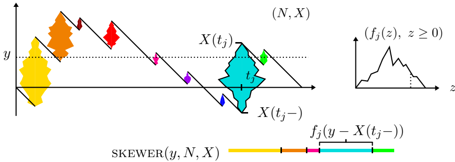
FIG 1.1. Left: The slanted black lines comprise the graph of the scaffolding X . Shaded blobs decorating jumps describe spindles: points (t_j, f_j) of N . Right: Graph of one spindle. Bottom: A skewer, with blocks shaded to correspond to spindles; not drawn to scale.
