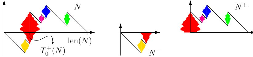
FIG 1.2. Decomposition of a bi-clade around the middle mass, m_0 .
