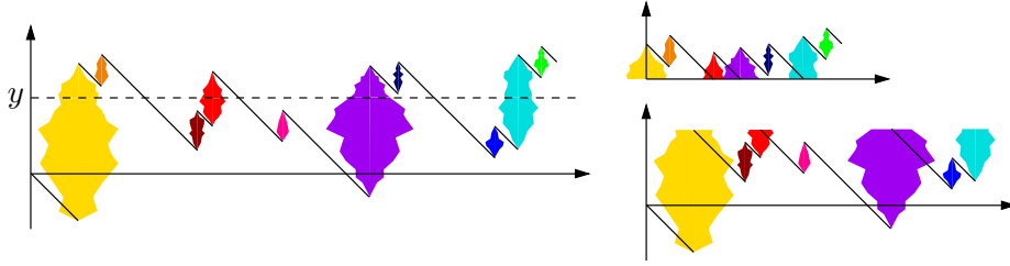
FIG 4.2. Left: (N, \xi(N)) . Right: (\text{CUTOFF}^{\geq}(y, N), \text{CUTOFF}^{\geq}(y, \xi(N))) (above) and (\text{CUTOFF}^{\leq}(y, N), \text{CUTOFF}^{\leq}(y, \xi(N))) , as in (4.16).
